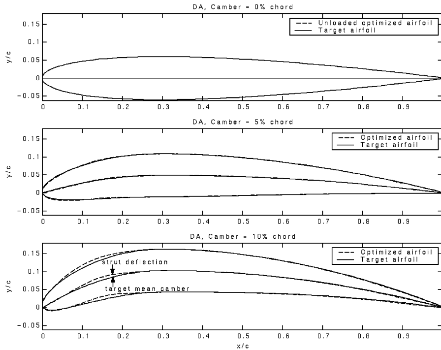
Fig. 3 Baseline plus target and computed airfoils for morphing-optimized beam (DA).
