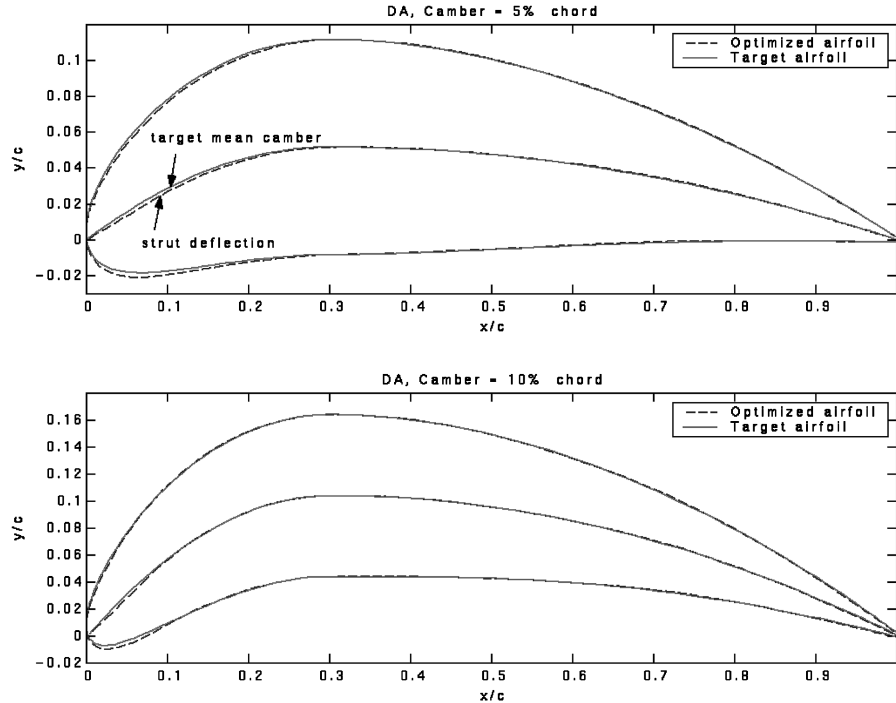
Fig. 11 Target and computed airfoils for morphing-optimized beam after CFD-based optimization.
