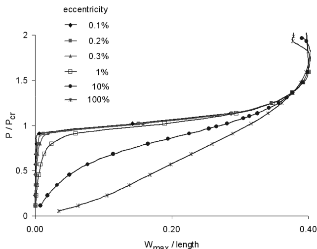
Fig. 2 Sensitivity of regular struts to eccentricity of loading.
