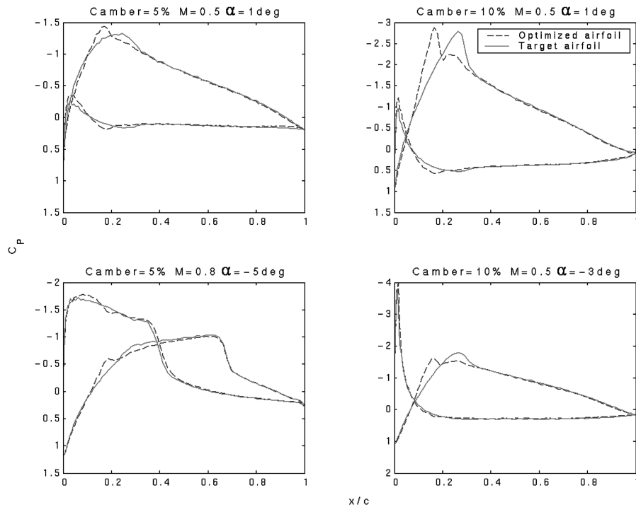
Fig. 8 Pressure distributions for morphed and target cambered airfoils, under mild and more severe flows.
