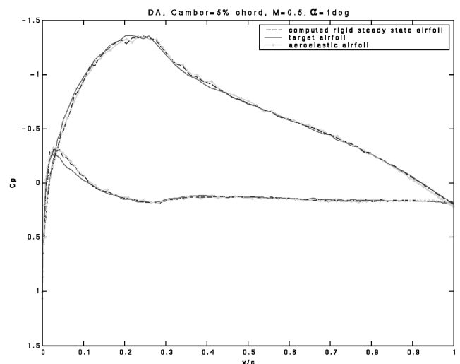
Fig. 10 Pressure distributions for aerodynamically loaded, morphed, and target cambered airfoils.
