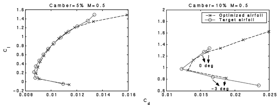
Fig. 9 Drag polars for different cambers.
