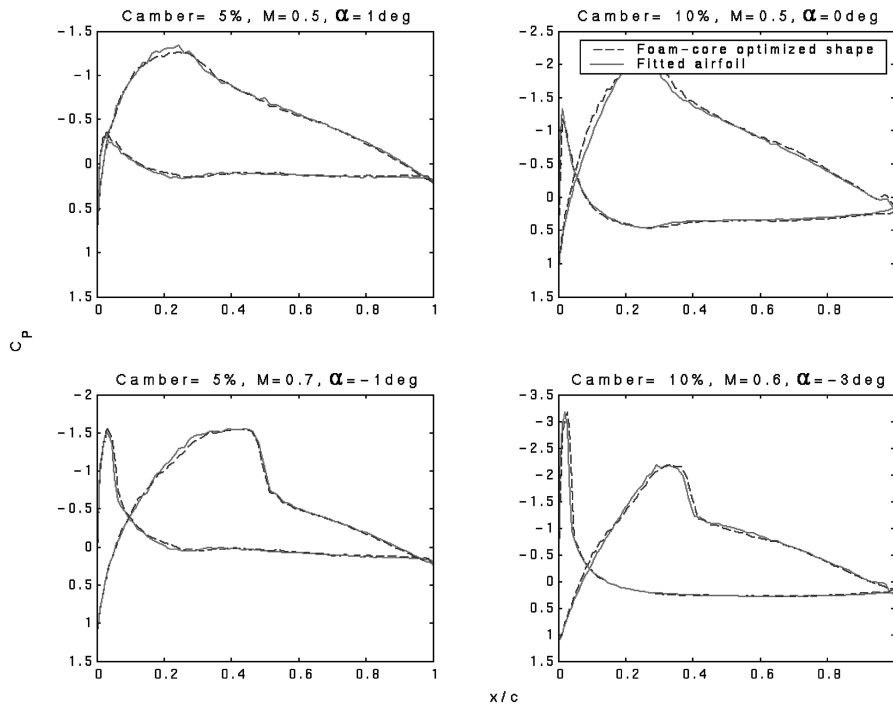
Fig. 15 Pressure plots for foam core model of morphed airfoils.
