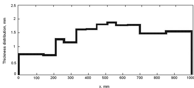
Fig. 4 Morphing-optimized beam (DA): semithickness.
