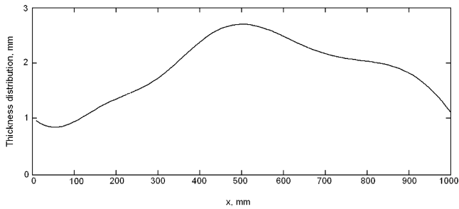
Fig. 6 Morphing-optimized beam (NURBS): semithickness.
