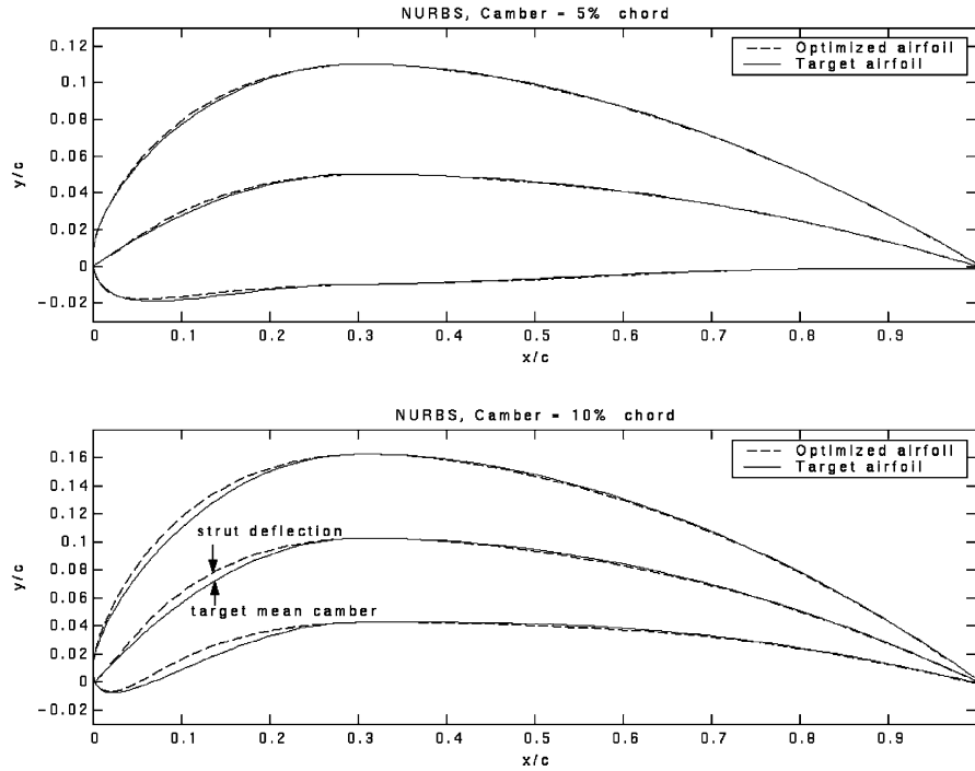
Fig. 5 Target and computed airfoils for morphing-optimized beam (NURBS).
